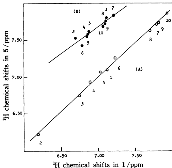
Fig. 2. Correlation between ^1\text{H} chemical shifts in 5 and 1 ; numbering as in Table 1. A, \delta_4(5) vs. \delta_3(1) . B, \delta_3(5) vs. \delta_4(1) .
